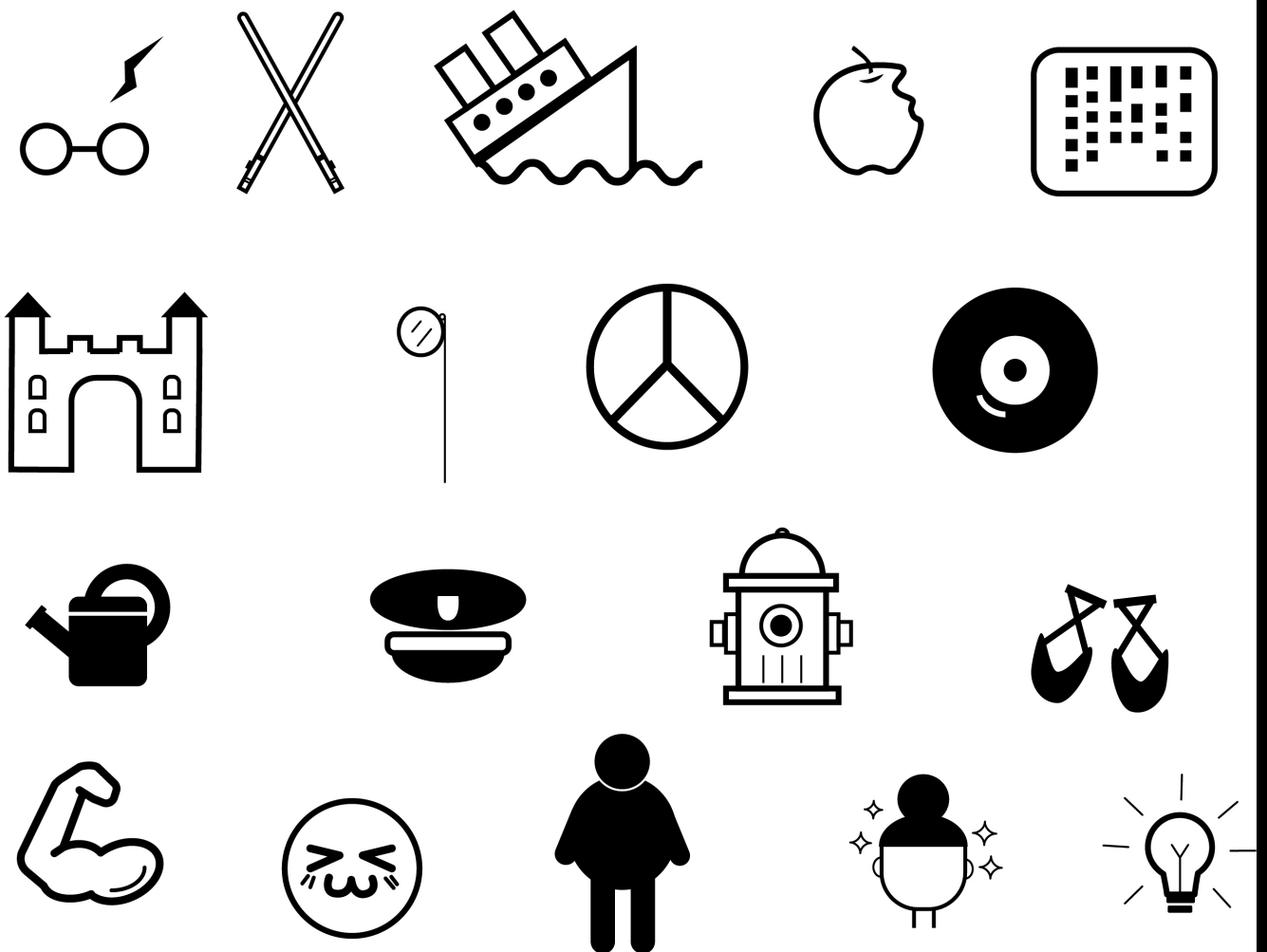
2D icons
